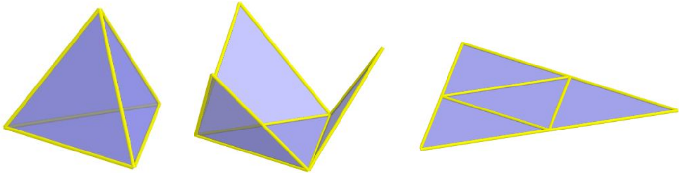
Triangular Pyramid
