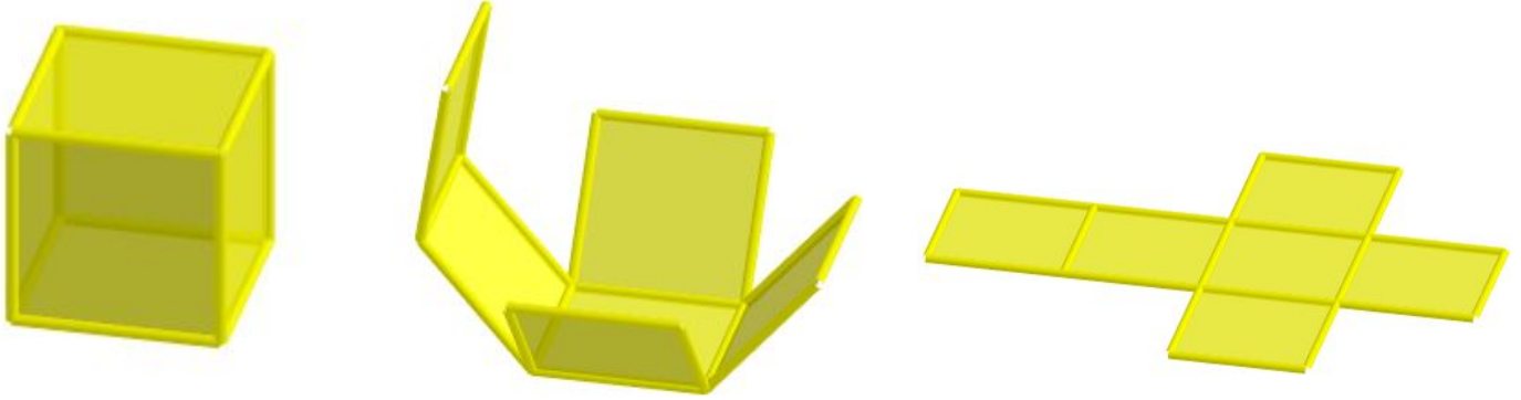
Rectangular Prism
