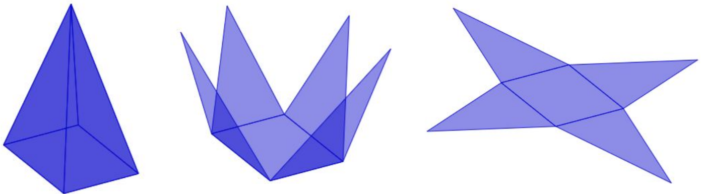
Rectangular Pyramid
