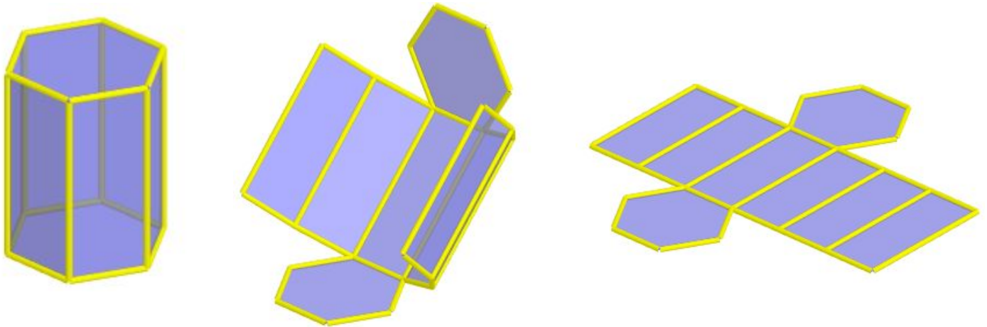
Hexagonal Prism
